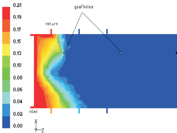
(a) Oxygen distribution – base case
