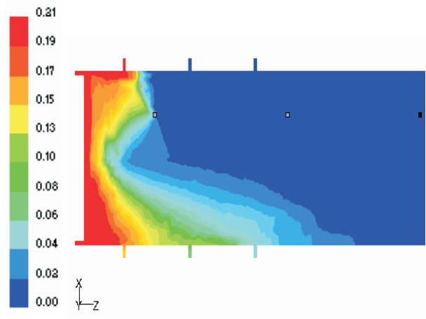
(b) Oxygen distribution – open intake case
