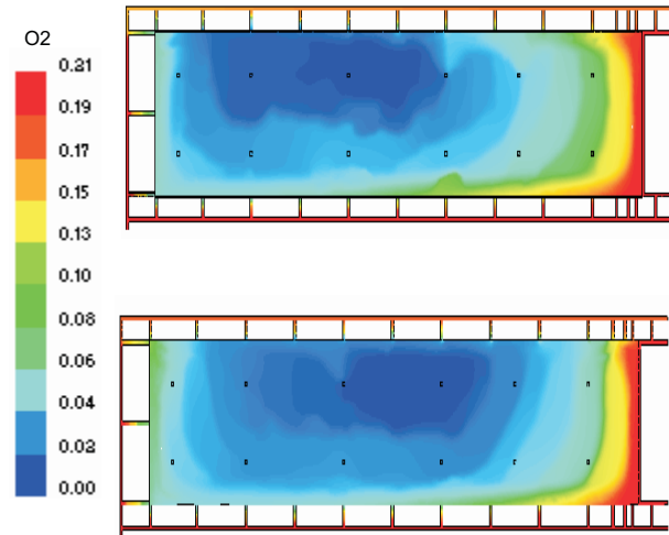
(b) Oxygen distribution
