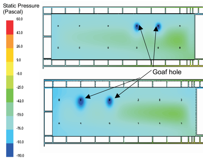
(a) Static goaf gas flow pressure
