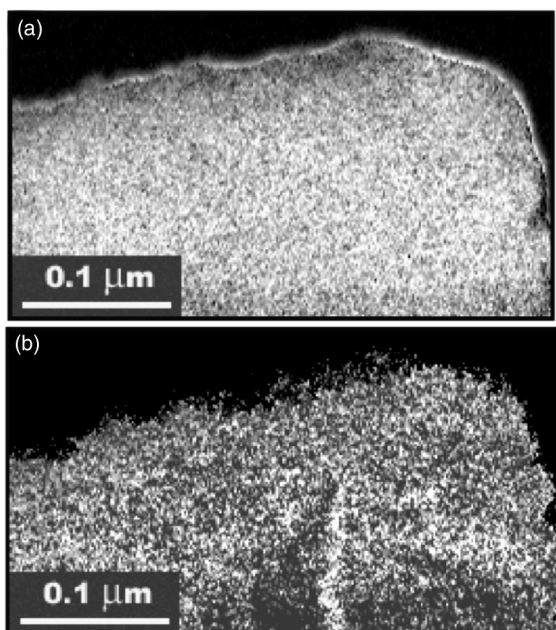
Figure 2. EDS element mapping of (a) Fe (b) P in \text{LiFePO}_4 compound.
