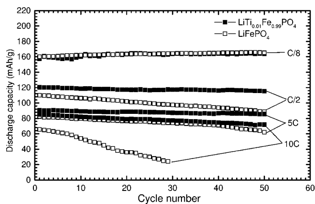
Figure 6. Discharge capacity vs. cycle number at different charge/discharge rates for \text{LiFePO}_4 and \text{LiTi}_{0.01}\text{Fe}_{0.99}\text{PO}_4 electrodes.
