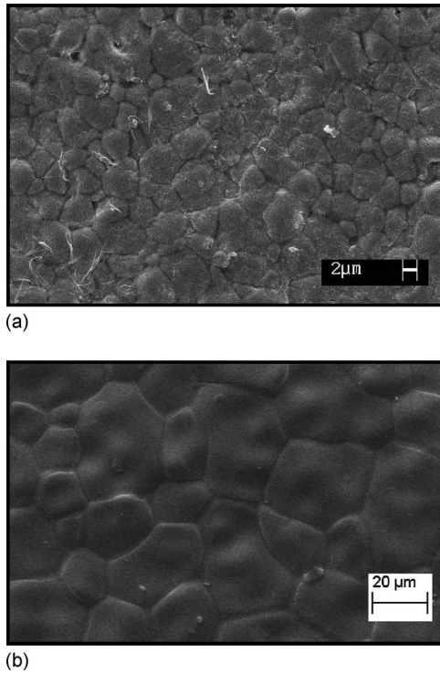
FIG. 3. SEM micrograph of (a) \text{La}_{0.7}\text{Ca}_{0.2}\text{Sr}_{0.1}\text{MnO}_3 and (b) \text{La}_{0.7}\text{Ca}_{0.2}\text{Sr}_{0.1}\text{MnO}_3:\text{Ag}_{0.2} .
