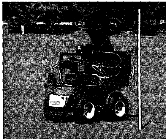
Figure 1: Titan 4-wheel drive robot navigating across a field using poles as landmarks.
