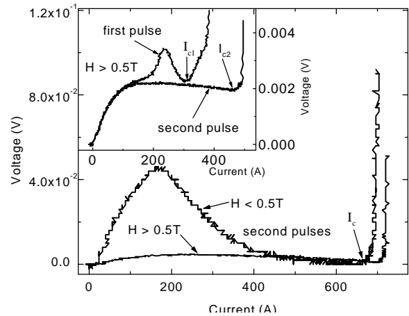
Figure 1: Typical voltage-current characteristics for an iron-sheathed MgB_2 wire at two different fields H, for second current pulse after changing H. The peak at low currents occurs for H < 0.5T . Inset: typical V-I for H > 0.5T . The peak at low currents often occurs in the first pulse of the current after H was changed. There is no peak for the subsequent current pulses.
