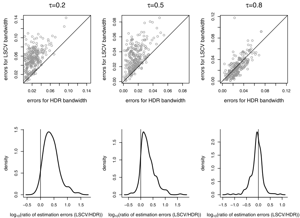
FIG. 3. Summary of simulation comparison between \hat{h}_{\tau\text{-HDR}} and \hat{h}_{\text{LSCV}} for \tau = 0.2, 0.5 and 0.8 and 250 samples of size 1000 generated from Density 4 of Marron and Wand (1992). The upper panels are scatterplots of the errors \mu_f(\hat{R}_{h,\tau}\Delta R_\tau) for h = \hat{h}_{\text{LSCV}} on the vertical axes and h = \hat{h}_{\tau\text{-HDR}} on the horizontal axes. The lower panels are kernel density estimates of \log_{10}((\text{error for } h = \hat{h}_{\tau\text{-HDR}})/(\text{error for } h = \hat{h}_{\text{LSCV}})) .
