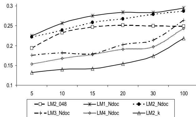
Fig. 2. Cut Off Diagram of LM1-4, Lnu.Itu and Lnc.btc.
