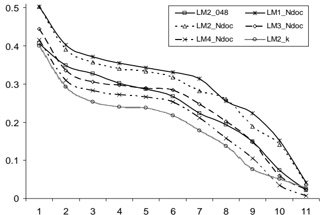
Figure 1: Precision- Recall Graph for language models LM1 to LM4 with different tuning
