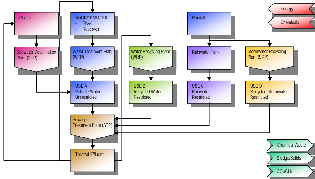
Figure 2 Water, wastewater and stormwater cycle with recycling options
