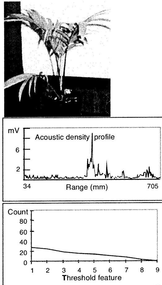
Fig. 10. Image, acoustic density profile, and threshold curve averaged over 360^\circ for a class d) plant: Rhopalostylis baneri .
