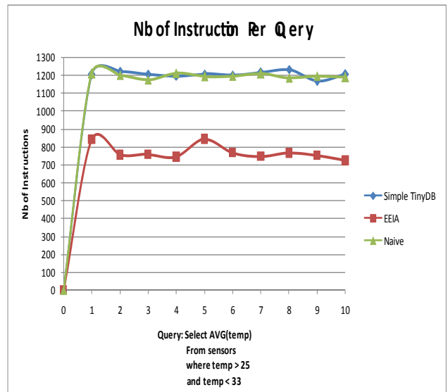
Fig. 7 Nb of instructions per query
