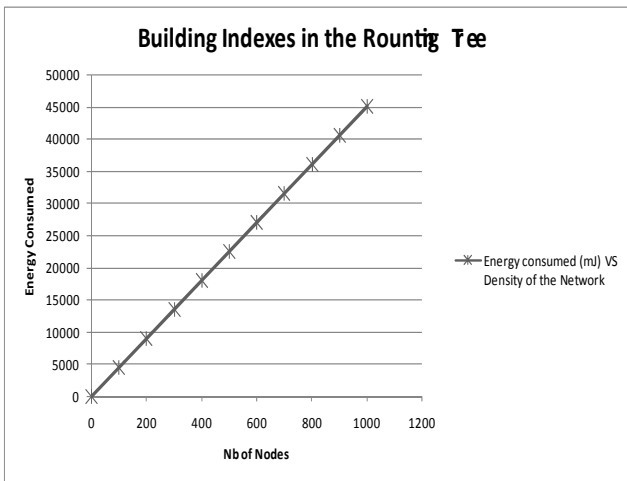
Fig. 4 Building the routing tree
