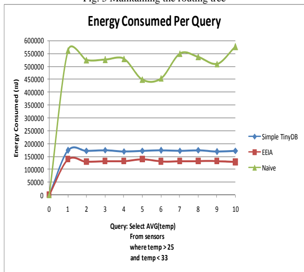
Fig. 6 Energy consumption per query
