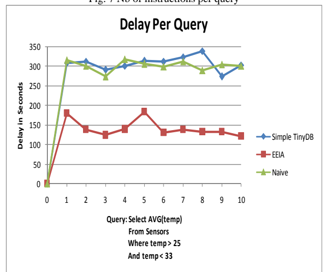
Fig. 8 Time delay per query
