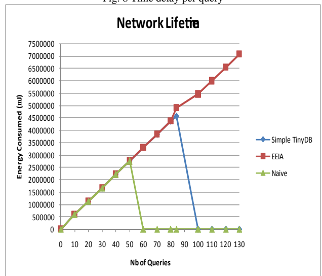
Fig. 9 Network lifetime
